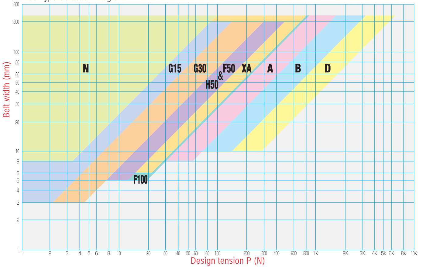
Belt Type Selection Diagram
